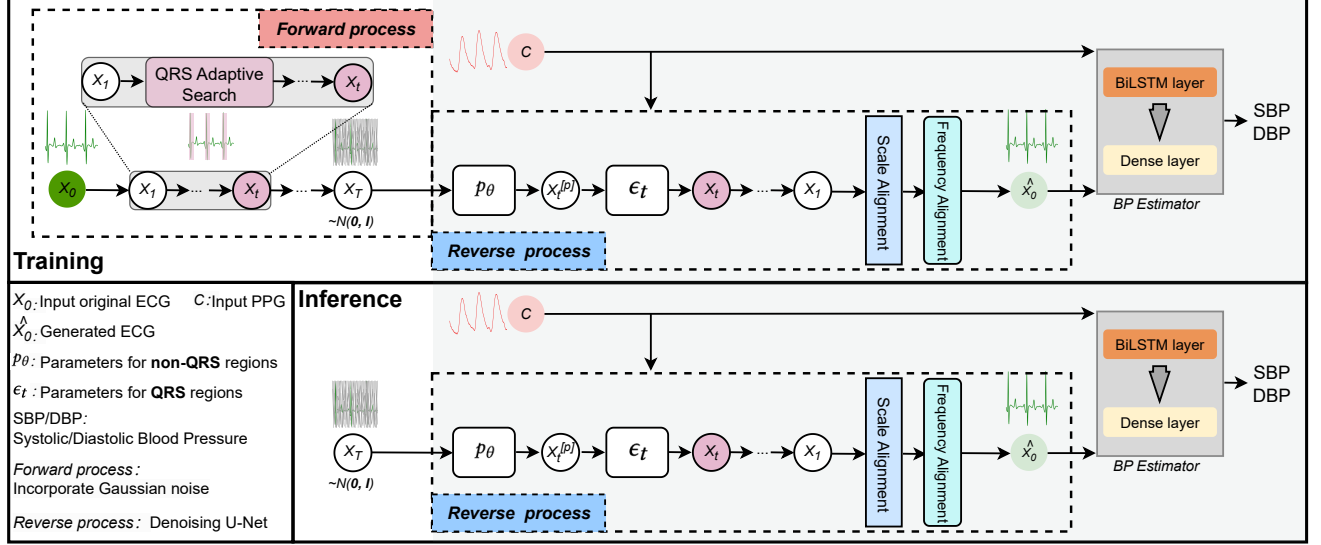
Figure 6: Overview of the proposed PPG framework for blood pressure monitoring.
