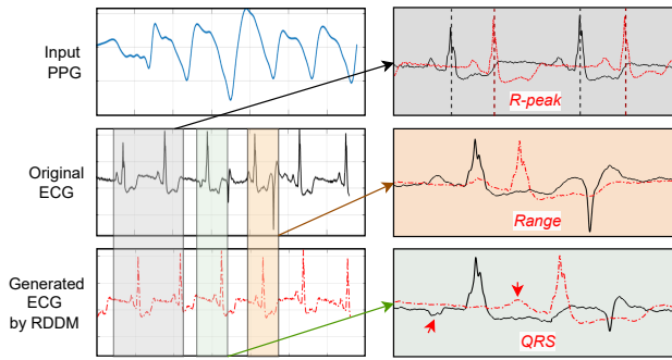
Figure 2: The ECG generated by RDDM exhibits limitations in signal fidelity: misalignment of R-Peak, variability in amplitude, and distortions in QRS waveform.
