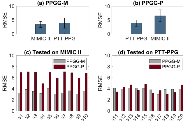
Figure 8: Results of cross-dataset validation.
